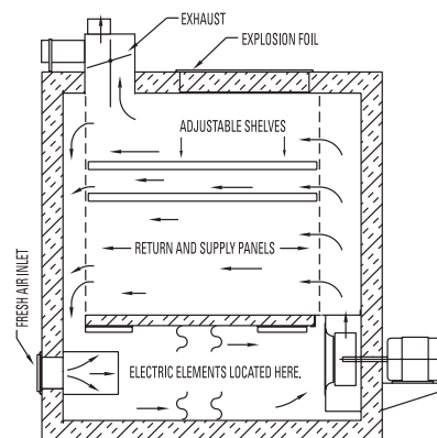
RFF front view cross section showing airflow pattern.
